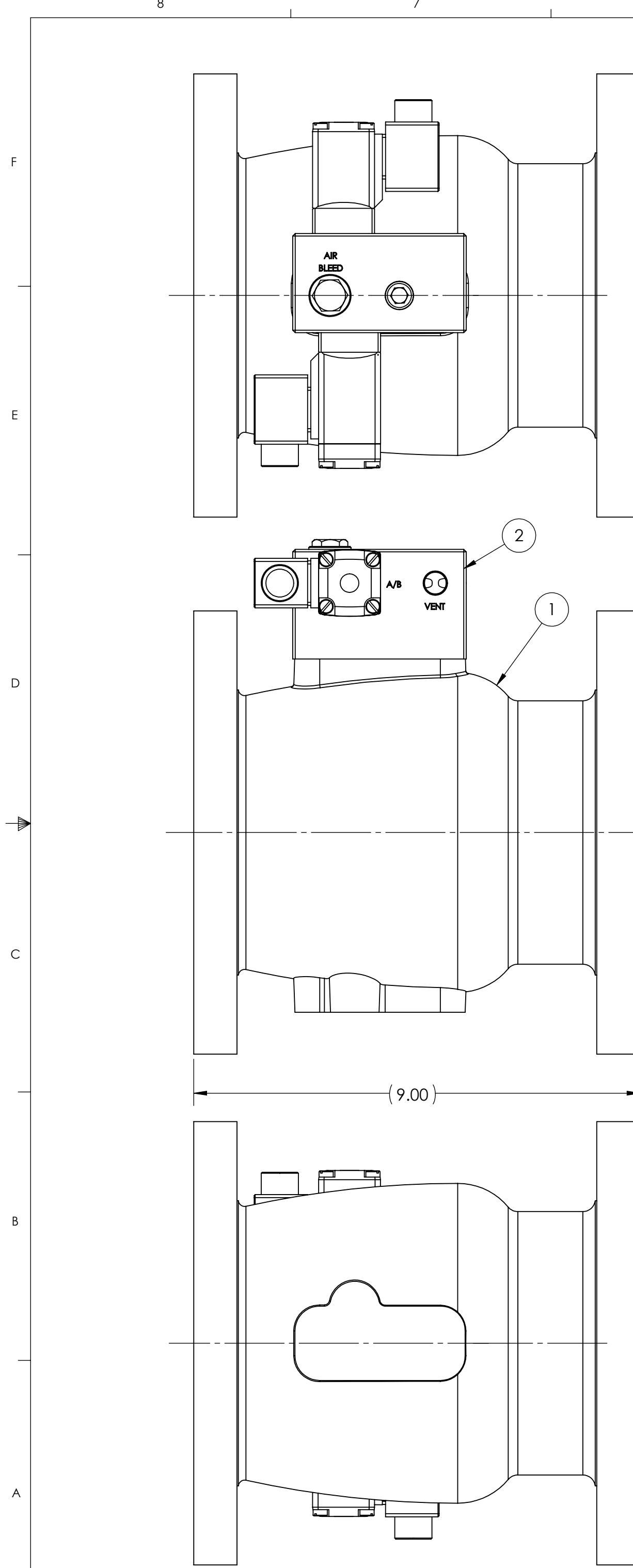
P/N PCV286FF SHOWN
