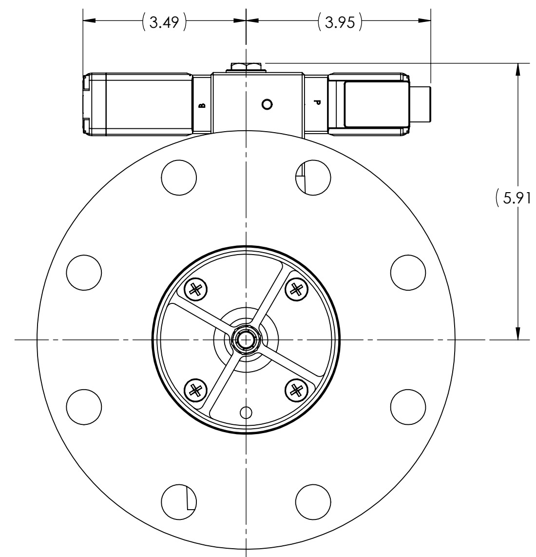
P/N PCV286FF SHOWN
